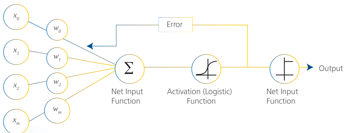
Fig 1: Logistic Regression
