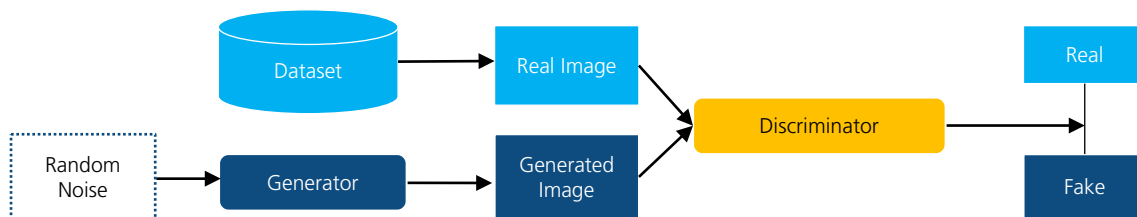
Figure 1: GAN architecture
